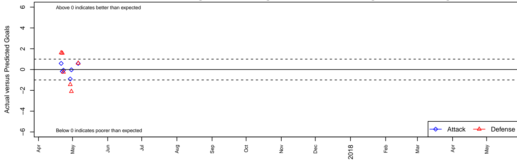
Wenatchee FC B B05 Dots are actual minus expected GF (blue circles) and GA (red triangles). Blue line is smoothed change in attack strength. Red is smoothed change in defense strength.
